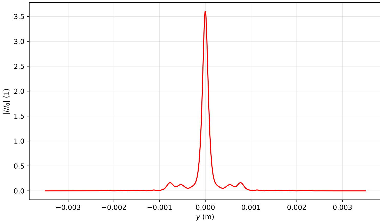
Intensity profile I(x=0, y, z=1.194)/I_0 , P_{in}=8.5P_{cr} , artificial time
